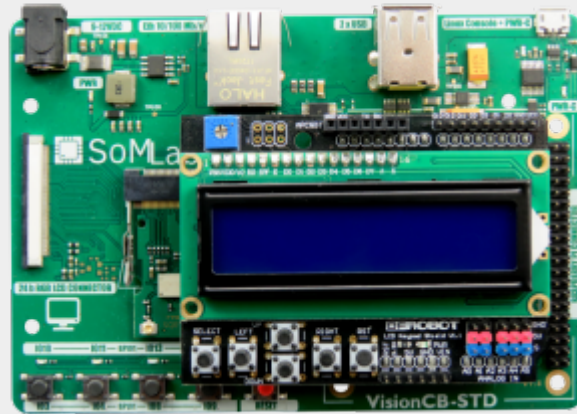
VisionCB-STD board with Arduino Shield
